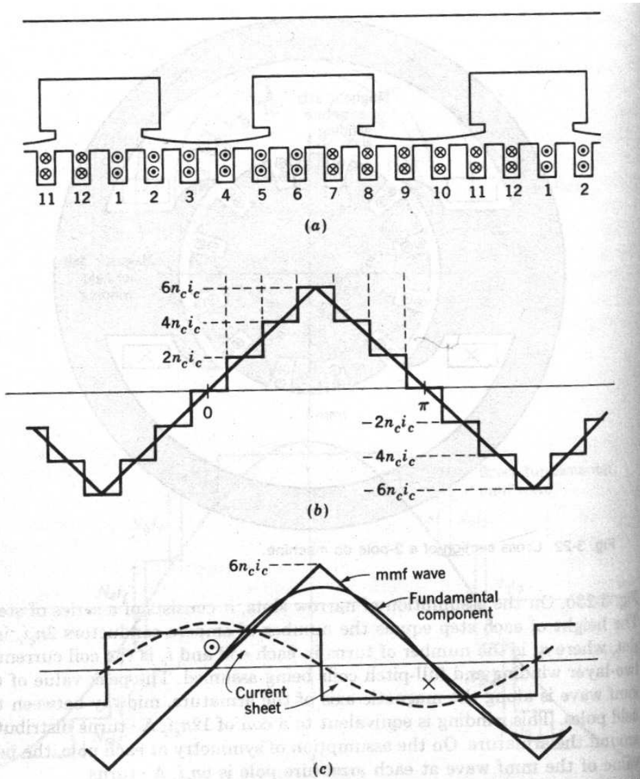
Fig. 3-23. (a) Developed sketch of the dc machine of Fig. 3-22, (b) mmf wave, (c) equivalent sawtooth mmf wave, its fundamental component, and equivalent rectangular current sheet.
